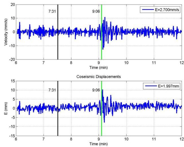
Fig.7 Velocity and coseismic displacement time series of station XJKC, 250 Km away from epicenter
