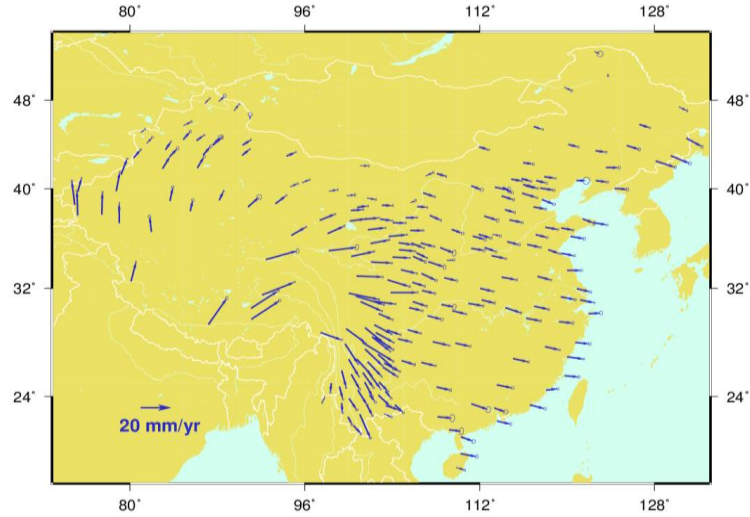
Figure 2. CMONOC GPS result of the horizontal velocity field of continental China respect to EURA The arrows represent the velocities. The ellipses represent the 95% confidence level.
