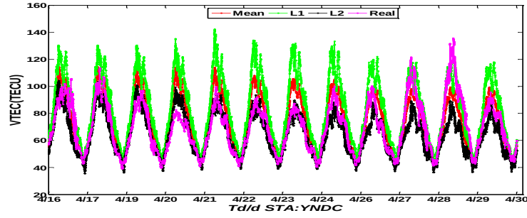
Fig.4 Time series of VTEC for 4 stations during the Lushan earthquake, where “mean” refers to the VTEC median over the same epoch of successive 15 days and “real” refers to real-time VTEC observed at each epoch
