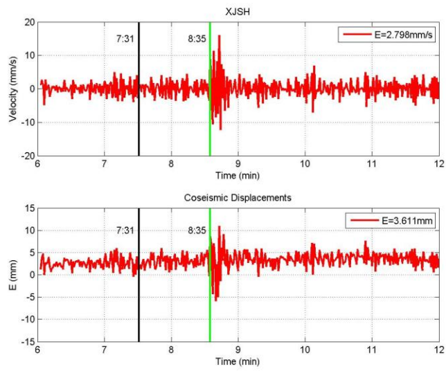
Fig.6 Velocity and coseismic displacement time series of station XJSH, 150 Km away from epicenter
