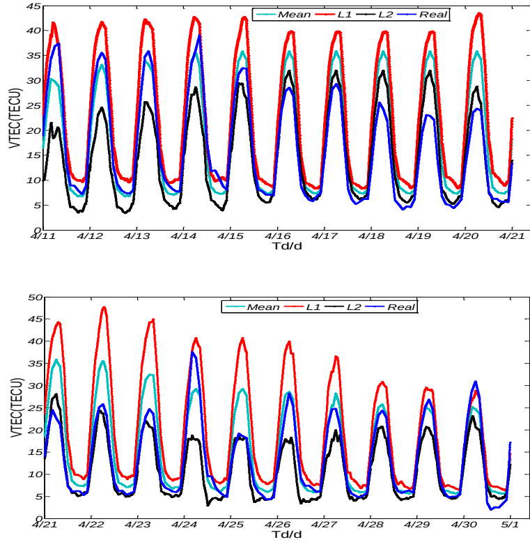
Fig.3 Time series of VTEC over the epicenter of Lushan earthquake, where “mean” refers to the VTEC median over the same epoch of successive 15 days and “real” refers to real-time VTEC observed at each epoch
