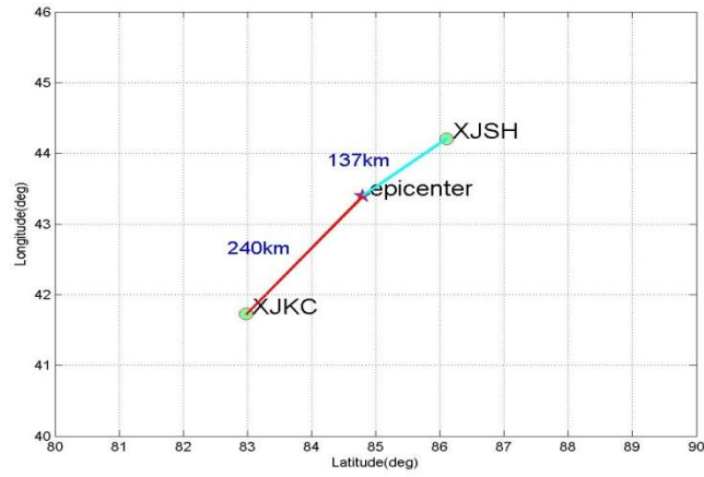
Fig.5 Plot of the epicenter and selected stations
